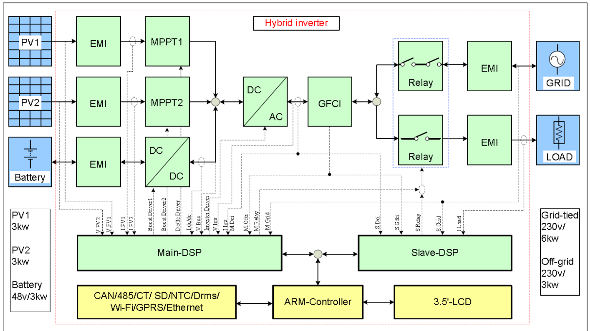
PGU Block Diagram:
